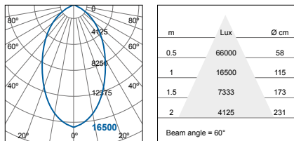
FHB71000v0-dc/ds+060D (150W) FHB71000v0-da+060D (150W)
