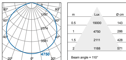
FHB71000v0-dc/ds+110D (90W) FHB71000v0-da+110D (90W)
