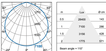
FHB71000v1-dc/ds+110D (125W) FHB71000v1-da+110D (125W)
