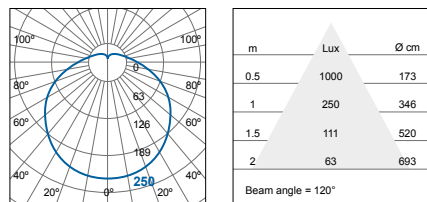
FCL71600v0-sc FCL71600v0-sc+LA10175 FCL71600v0-sc+LA11149
