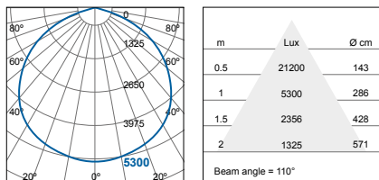
FHB71000v1-dc/ds+110D (90W) FHB71000v1-da+110D (90W)
