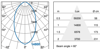
FHB71000v0-dc/ds+060D (125W) FHB71000v0-da+060D (125W)
