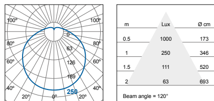
FCL71600v0 FCL71600v0+LA10175 FCL71600v0+LA11149
