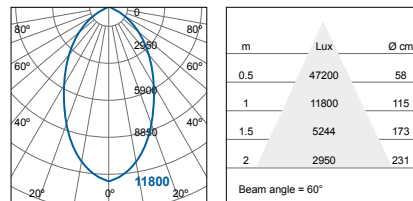
FHB71000v0-dc/ds+060D (100W) FHB71000v0-da+060D (1100W)
