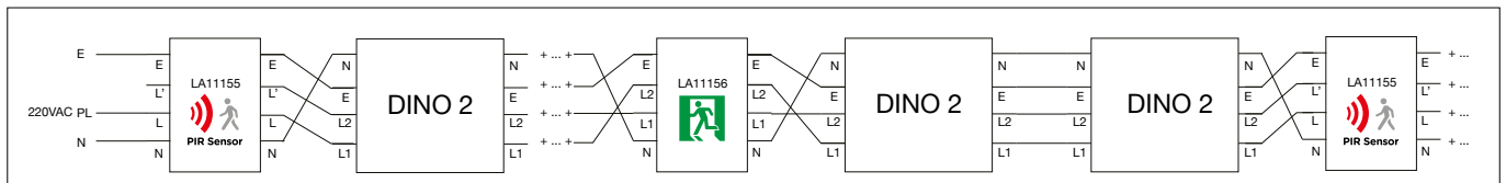
DINO 2 with PIR sensor module and Emergency module with Permanent live control only, especially for Tunnel or Underground car park application.
