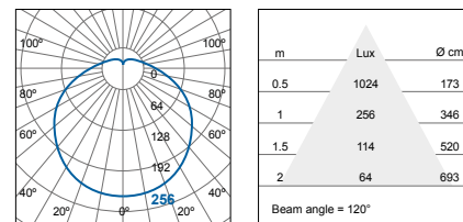
FCL71800v0-ds/sc FCL71800v0-ds/sc+LA10175 FCL71800v0-ds/sc+LA11149 FCL71800v0-ds/sc+LA10175+LA11149
