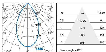
FLP70400v0-da/sc (29W)
