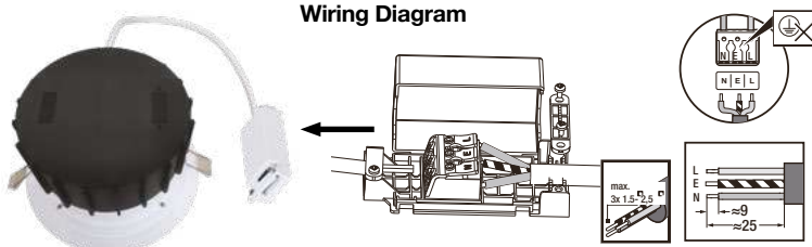
Wiring Diagram
