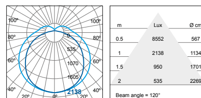
FOB80200v2-ds (70W)
