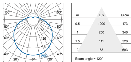
FCL72600v0-ds/sc FCL72600v0-ds/sc+LA10175 FCL72600v0-ds/sc+LA11149 FCL72600v0-ds/sc+LA10175+LA11149
