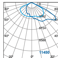
FFL74300v0-ds +060A135A-150W
