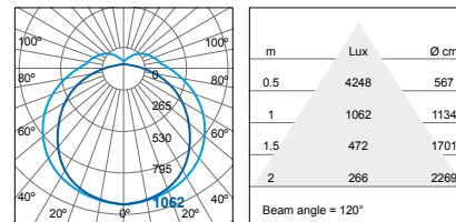
FOB80200v0-ds (33W)
