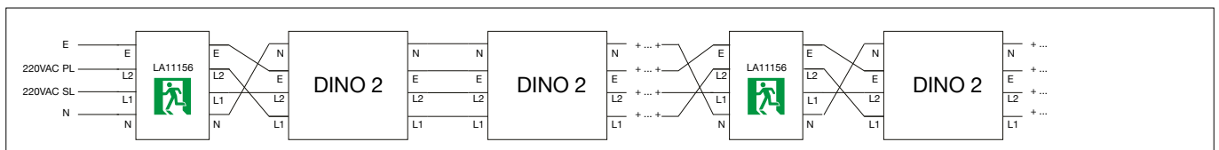
DINO 2 with Emergency module
